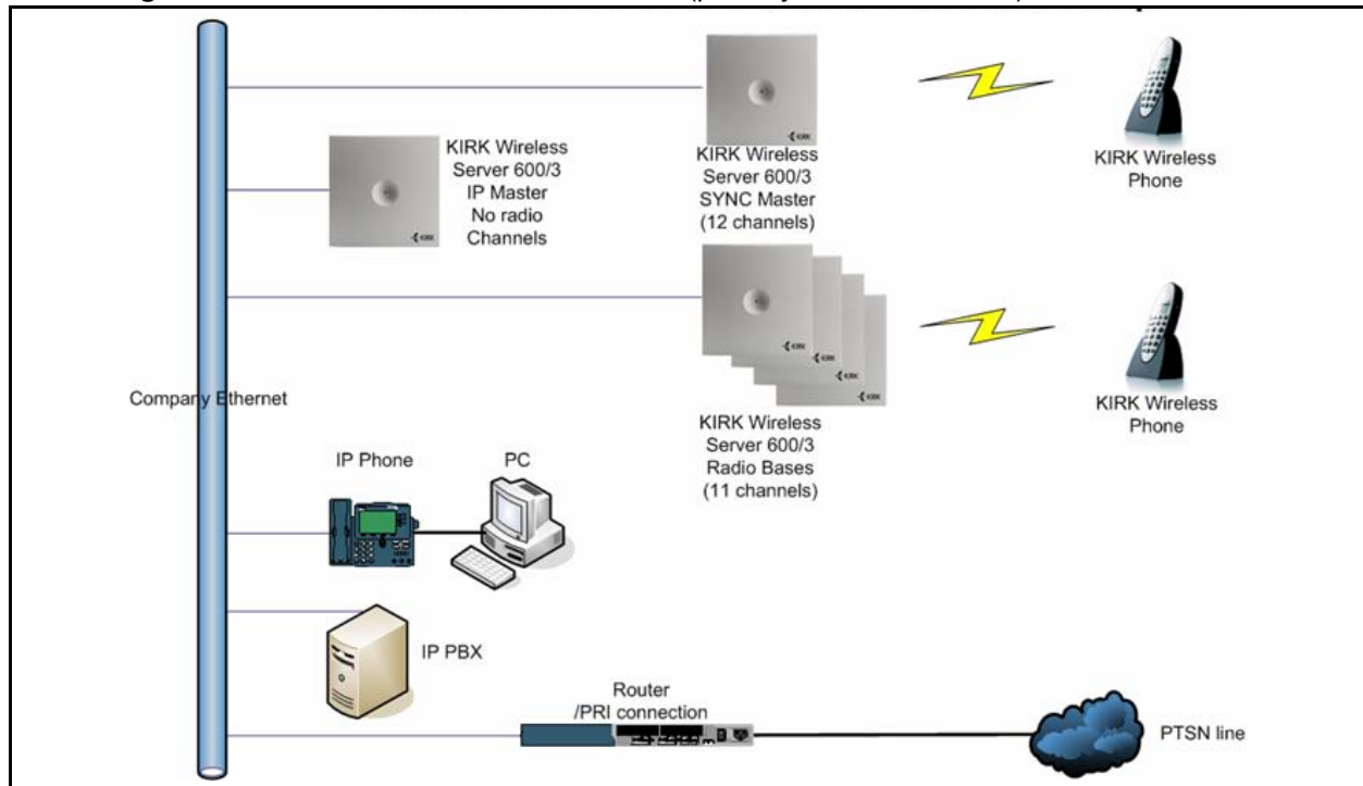
Figure 67 KWS600v3 Multi-cell installation (primary and secondaries)
